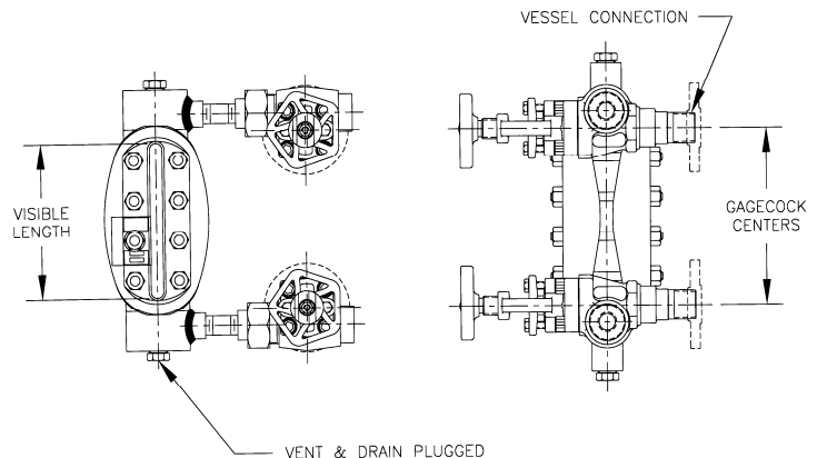
MODEL 720 GAGECOCK SHOWN
