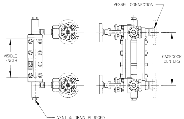
MODEL 520 GAGECOCK DIMENSIONS
