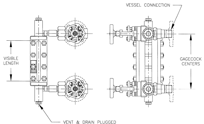
MODEL 520 GAGECOCK SHOWN
