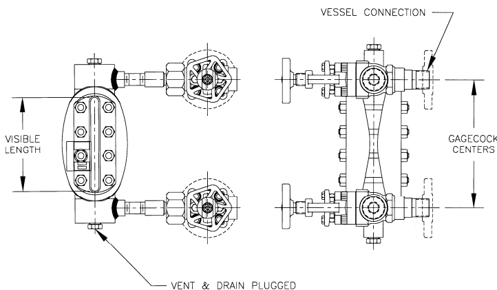
MODEL 520 GAGECOCK SHOWN
