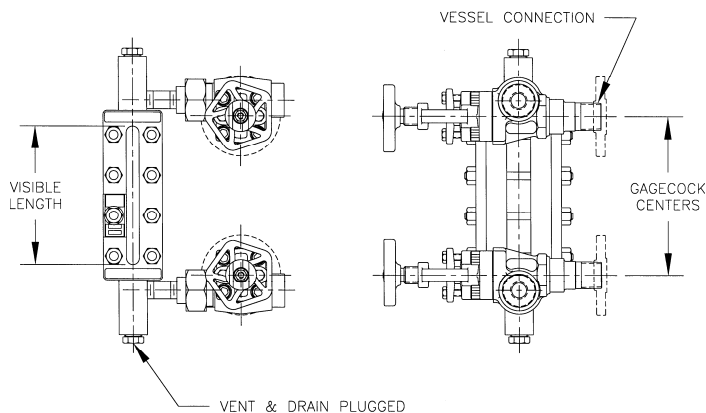
MODEL 720 GAGECOCK SHOWN
