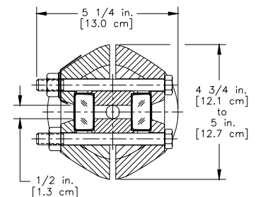
SECTION X-X (recessed chamber)
