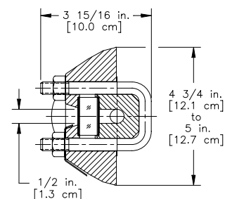
SECTION X-X (recessed chamber)
