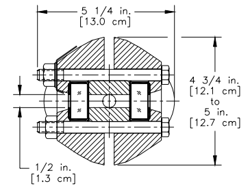
SECTION X-X (standard chamber)
