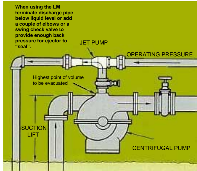
Priming centrifugal pumps
