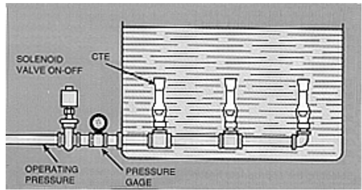
Heating liquids with Circulating Tank Educators (CTE)
