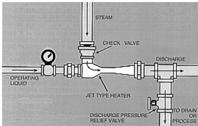
Typical in-line jet type heater installation
