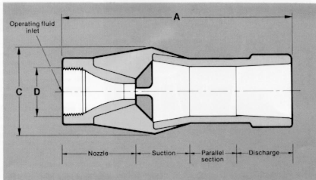
Cross section
